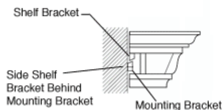
Step #3, Install shelf on mounting bracket
